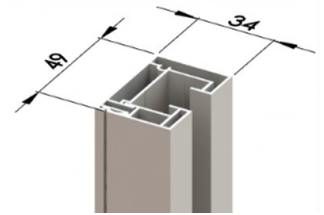
ZIP 100S
